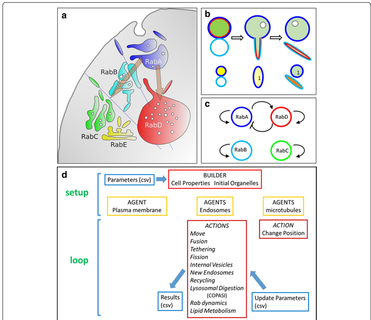
Fig. 1 Model description. a Informal model for transport along the endocytic route. Different Rab domains characterize four organelles: early endosomes (RabA), sorting endosomes (RabB), recycling endosomes (RabC), and late endosomes (RabD). A trans-Golgi network (TGN) is included as a RabE organelle for modeling transport of lysosomal enzymes (Figs. 7, 8 and 9). The straight lines represent microtubules that orientate the organelle movements. The brown arrows represent the movement of cargoes to recycling endosomes and to late endosomes/lysosomes. b Fusion and asymmetric fission. A RabA (blue perimeter) endosome carrying a membrane-bound cargo (red internal circle) and a soluble cargo (green content) fuses with an empty RabB (cyan) endosome. The hybrid vesicle has enough membrane to embrace the volume of the original endosomes, to form an internal vesicle, and to grow a tubule. When the tubule is separated from the round organelle, it carries the RabB domain, the red cargo and an amount of soluble cargo proportional to its volume. At the bottom, the way these organelles are representation in the model. The red and green contents are shown in the interior of the RabA organelle (yellow content). The color of the endosomes corresponds to the prevailing Rab in each organelle. After fusion, the resulting organelle is shown as an ellipse representing the ellipsoid with a size, and area/volume ration of the fused organelle. The color is set to blue because it is the prevailing Rab domain in the organelle. The interior is set to light yellow, because of the dilution of the green and red contents, and a "1" character is plotted indicating that the organelle carries an internal vesicle. After fission, the round organelle is represented as a circle with a blue perimeter, a "1" character (the internal vesicle), and a light green internal color, showing that part of the soluble content and all the membrane cargo went to the tubule. The tubule is represented by an elongated ellipse, with a cyan color corresponding to the RabB domain, and an orange interior representing the red content and part of the green content. c Informal representation of the Rab dynamics operating in the model (cut-out switch, [22]). Each Rab domain stimulates its own activation. In addition, RabA promotes RabD activation and RabD inhibits RabA activation. This dynamic was programmed in COPASI and the species, reactions, kinetic functions, and parameters are shown in Table 3. d Diagram of the simulation. Initially, Repast builds a set of organelles specified by parameters and characteristics read from a file (Additional file 1). The program then initiates an iterative loop where each agent is interrogated about performing or not a series of actions and changing its properties accordingly. The simulation records the evolution of the system and receives instructions from the user by periodically writing and reading external files (Additional file 2)
